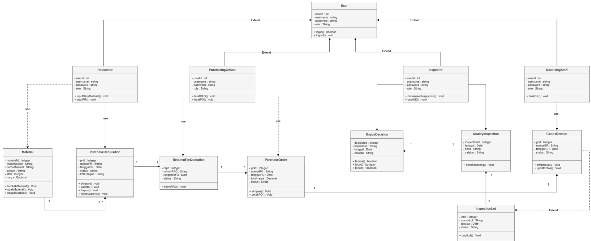
Gambar 3.3 Class Diagram Modul Material Management & Quality Management (MM/QM)
