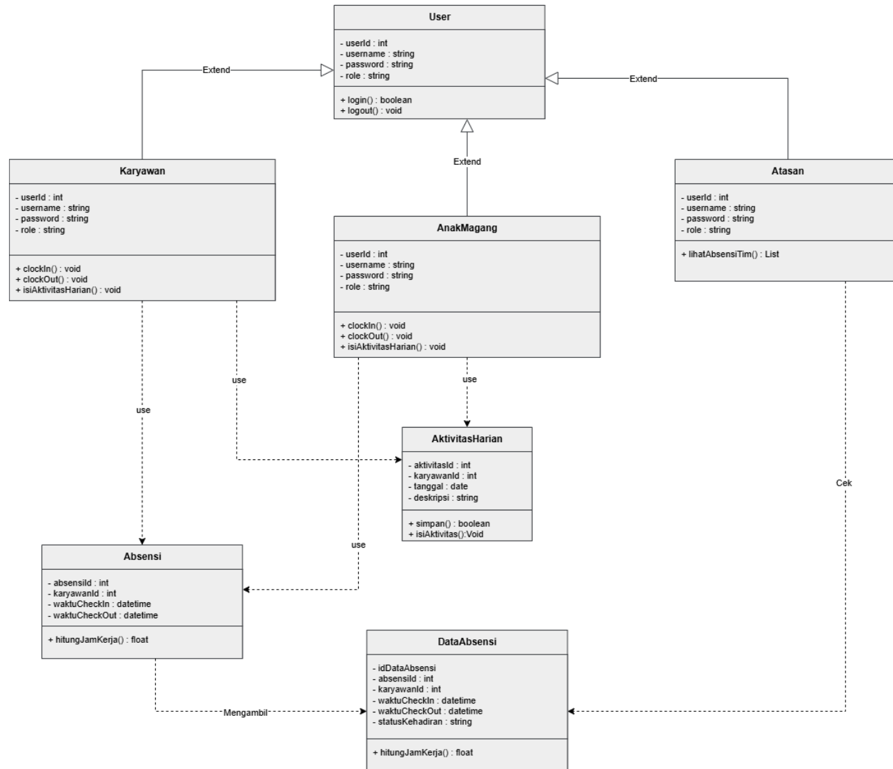
Gambar 3.1 Class Diagram Sistem Absensi
