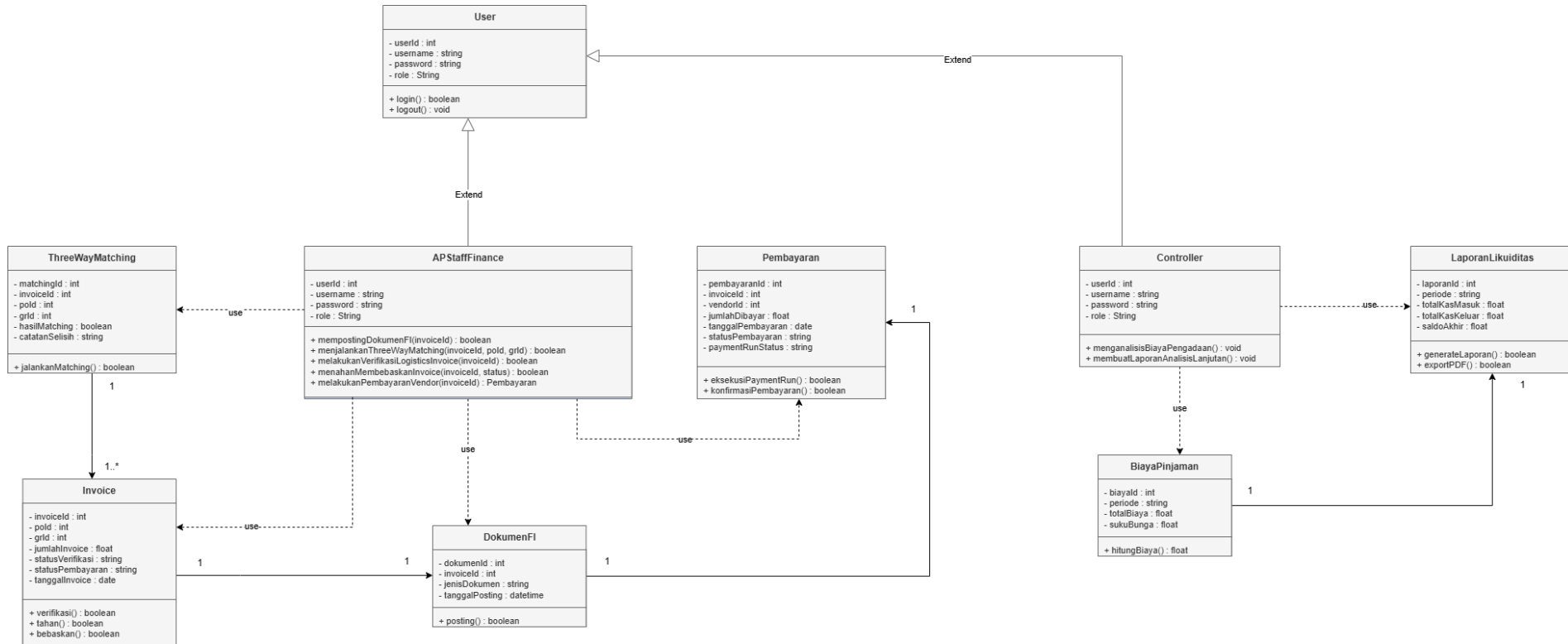
Gambar 3.5 Class Diagram Modul Financial Accounting & Controlling (FI/CO)
