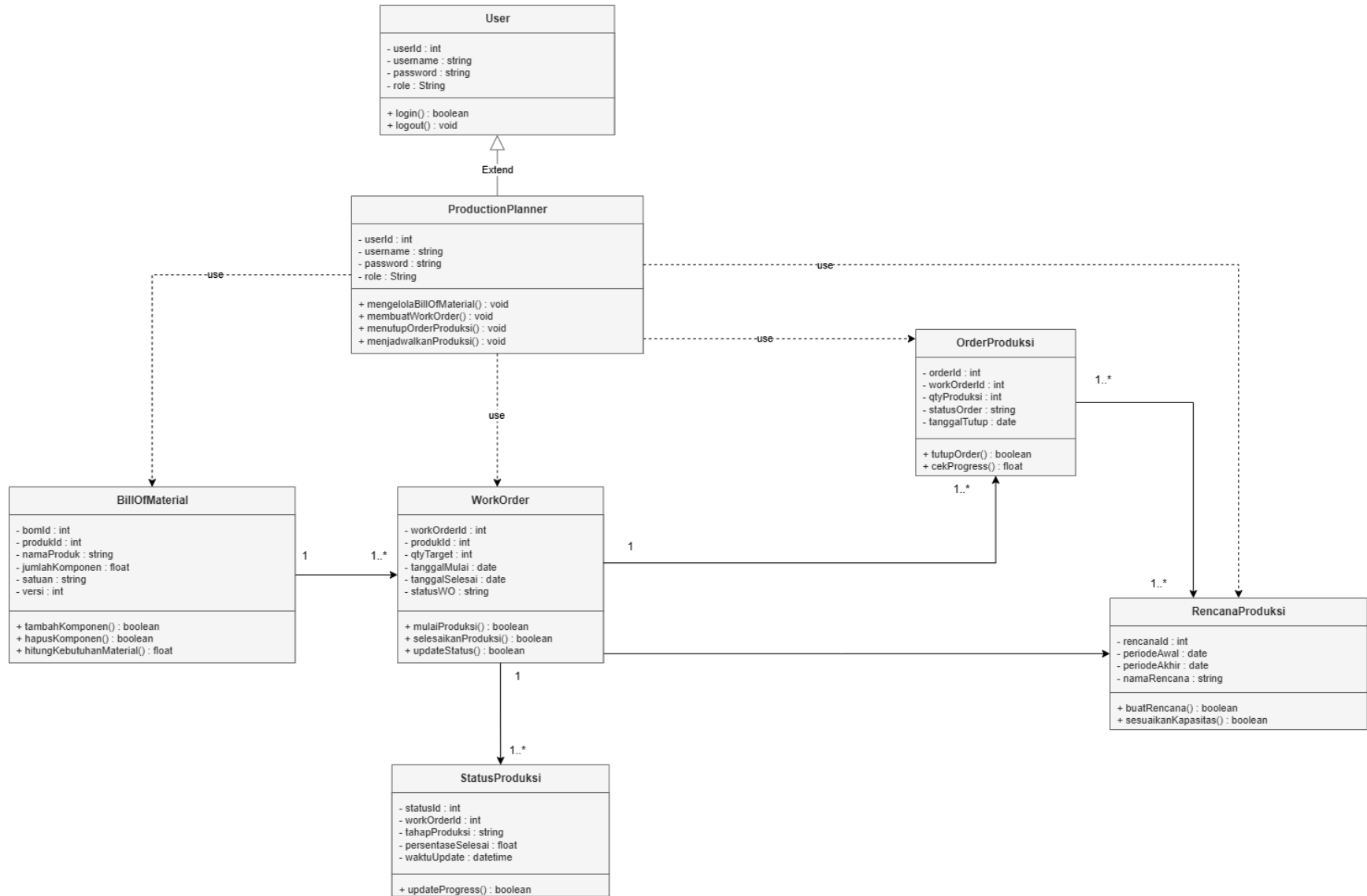
Gambar 3.6 Class Diagram Modul Production Planning (PP)
