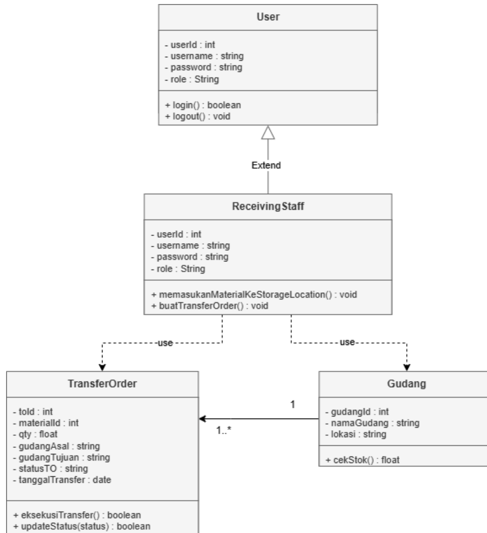
Gambar 3.4 Class Diagram Modul Warehouse Management (WM)
