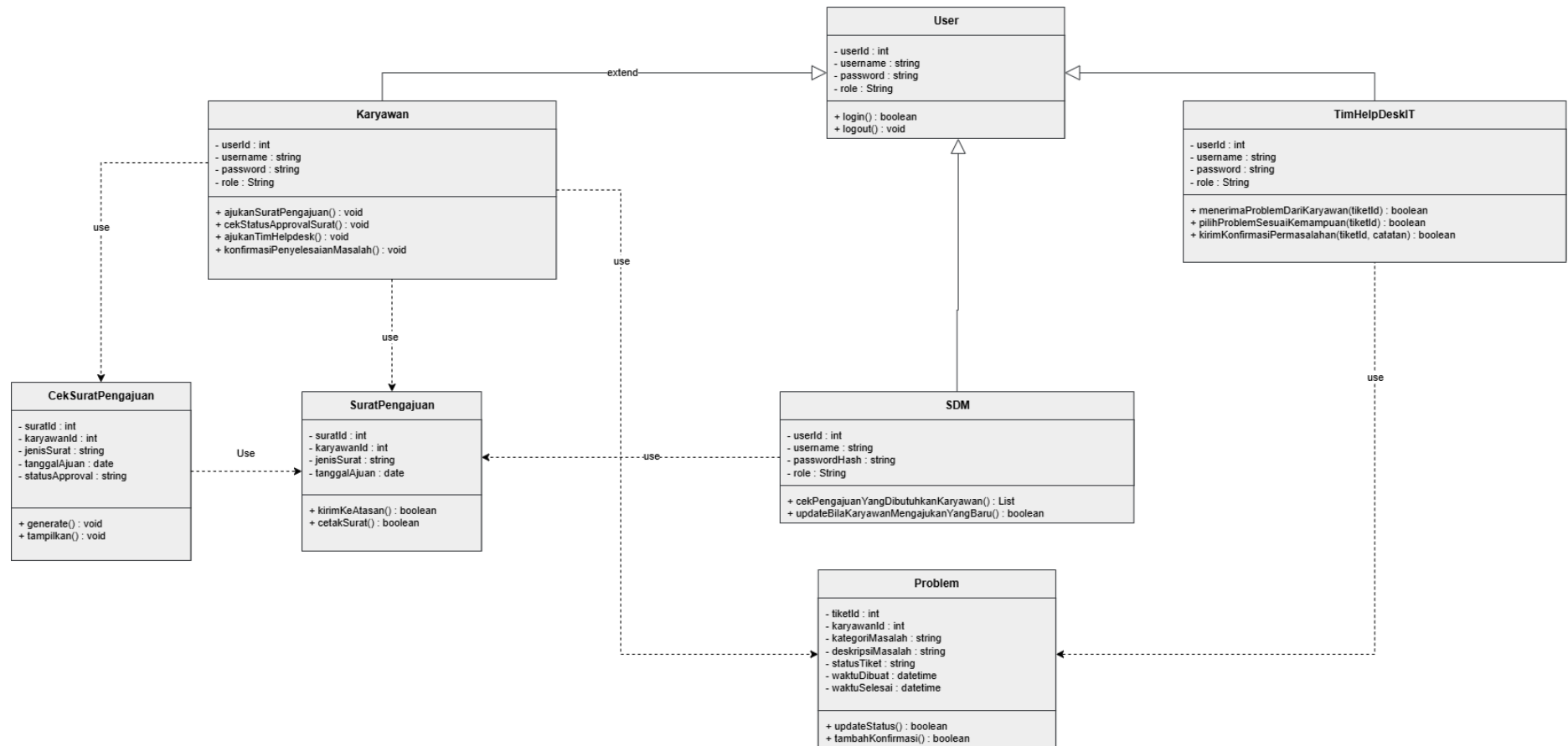
Gambar 3.2 Class Diagram Sistem Employee Self Service (ESS)
